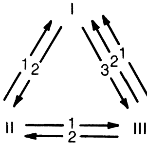
FIG. 5.—Fundamental equilibrium exchange pattern (model B)
