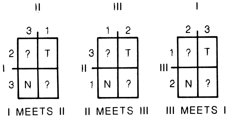
FIG. 1.—Trading matrices
