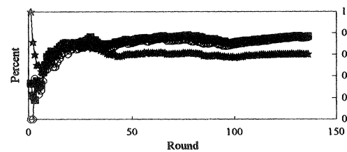
FIGURE 3. "BEST-RESPONSE" EFFICIENCY SCORES FOR MODEL A SESSIONS
