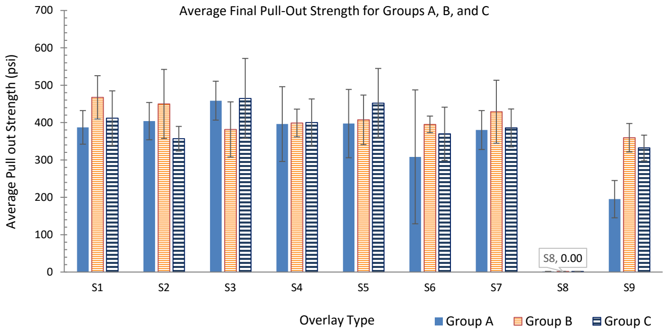
Figure 40. Average final pull-out strength for groups A, B, and C.
