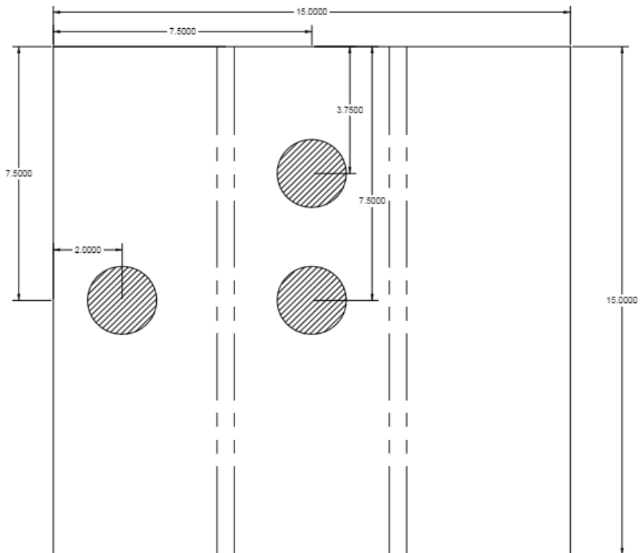
Figure 24. Schematic layout of sample coring locations after the end of exposure tests.
