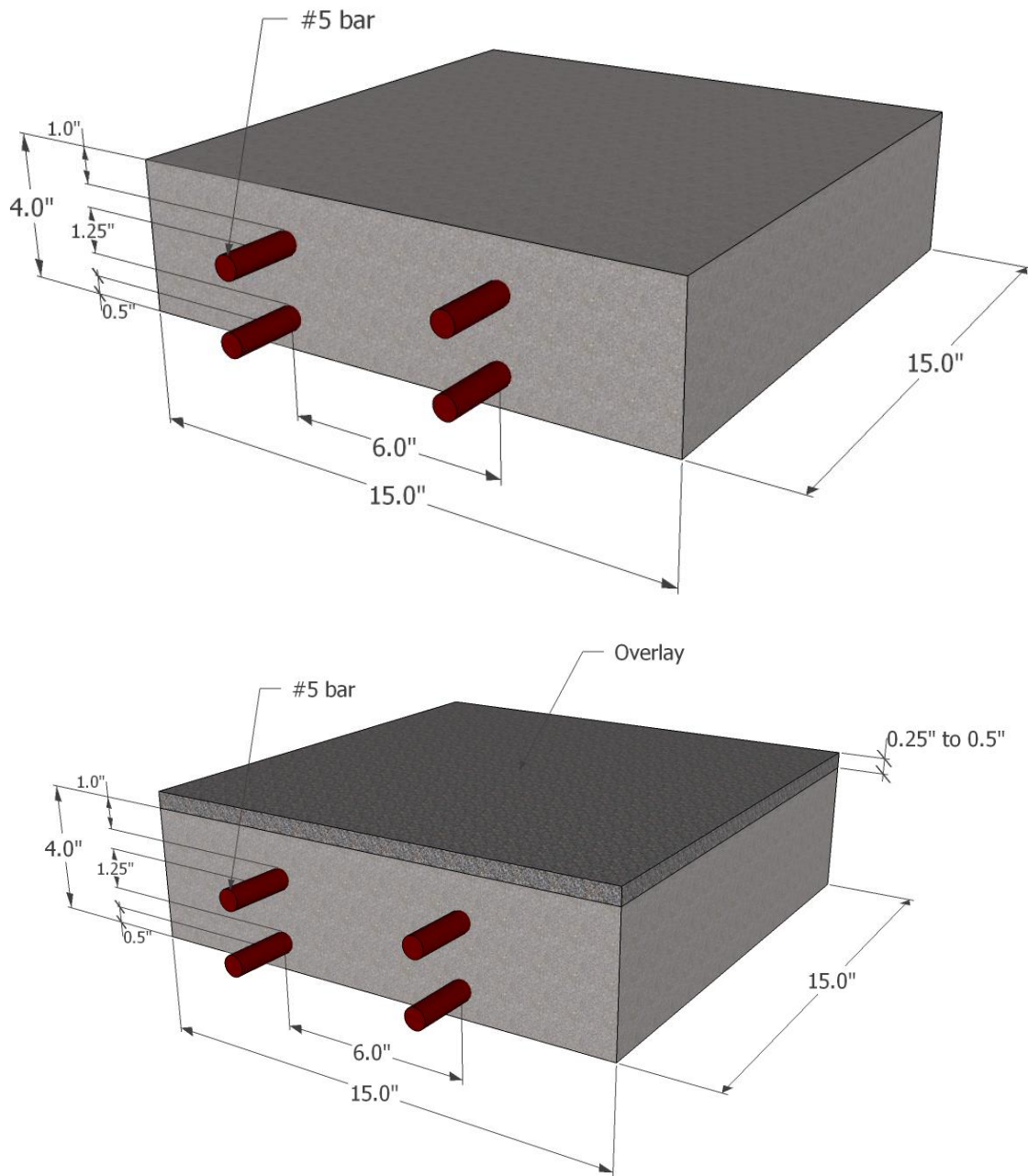
Figure 1. Concrete test specimen (with and without overlay).
