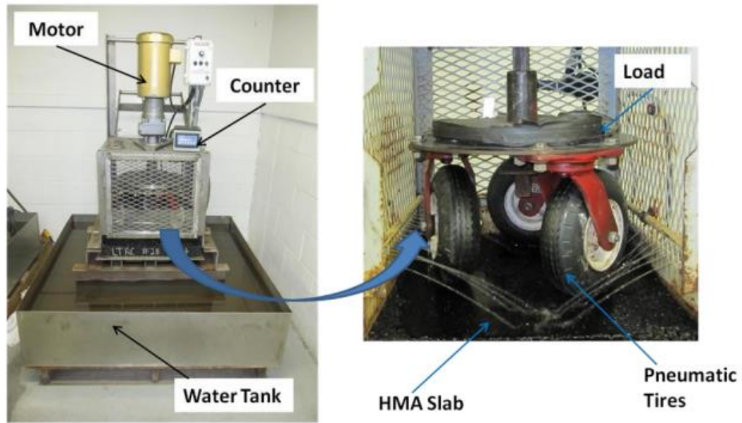
Figure 15. Three-Wheel Polishing Device (TWPD) developed by National Center for Asphalt Technology (NCAT) (Erukulla, 2011).
