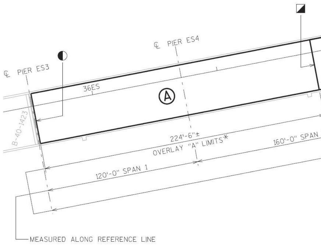
Figure 33. Section A drawing (from WisDOT).
