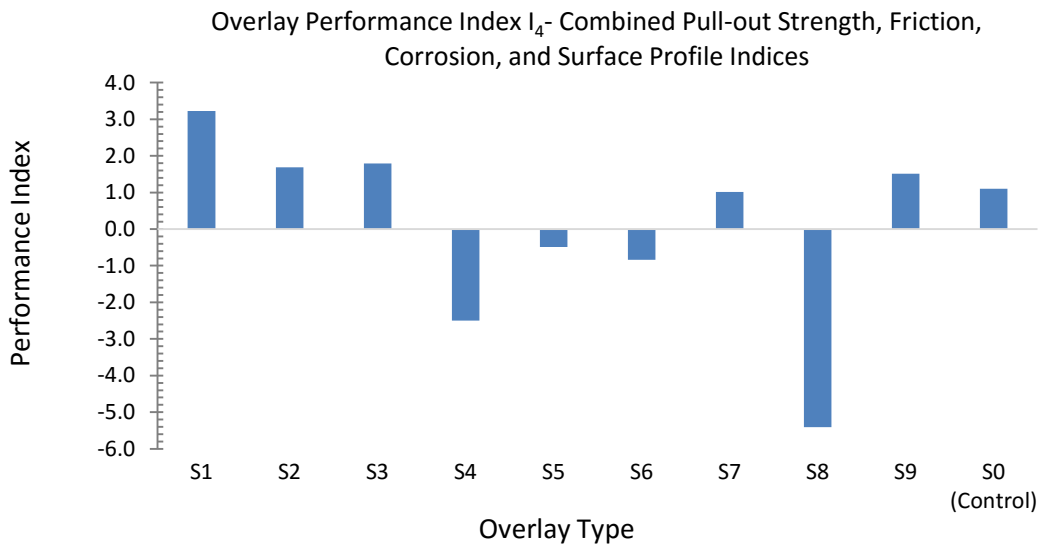
Figure 50. Overlay Performance Index ( I_4 ) - Combined pull-out strength, friction, corrosion, and surface profile indices.
