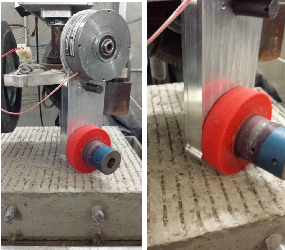
Figure 21. Friction measuring system for the UWM wear test machine.
