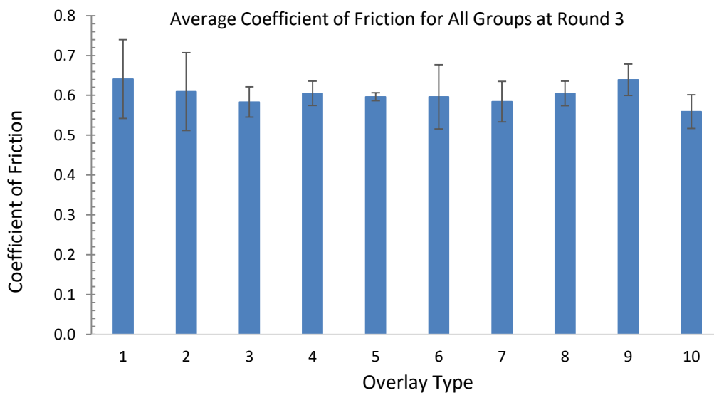
Figure 42. Average coefficient of friction for all groups at round 3.
