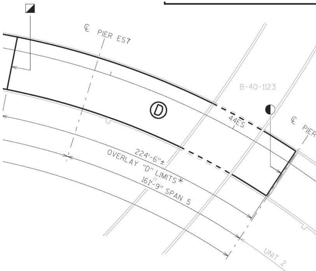
Figure 36. Section D drawing (from WisDOT).
