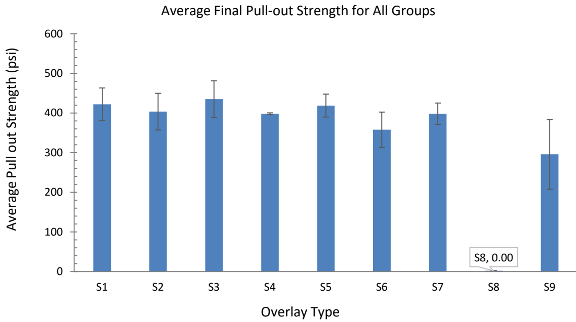
Figure 38. Average final pull-out strength of all groups.
