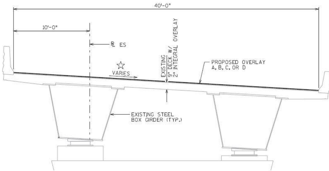
Figure 28. Cross section of Marquette Interchange ramp (from WisDOT project drawing).
