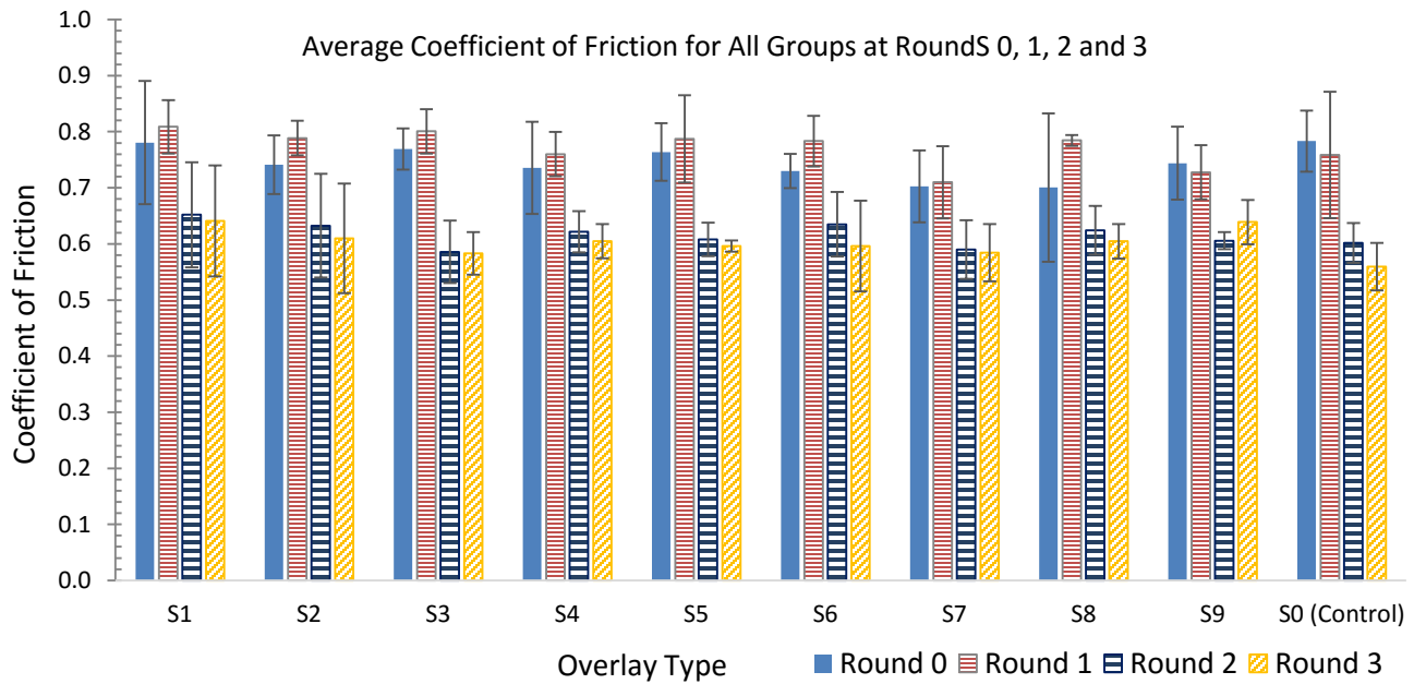
Figure 44. Average coefficient of friction for all groups at round 0, 1, 2, and 3.
