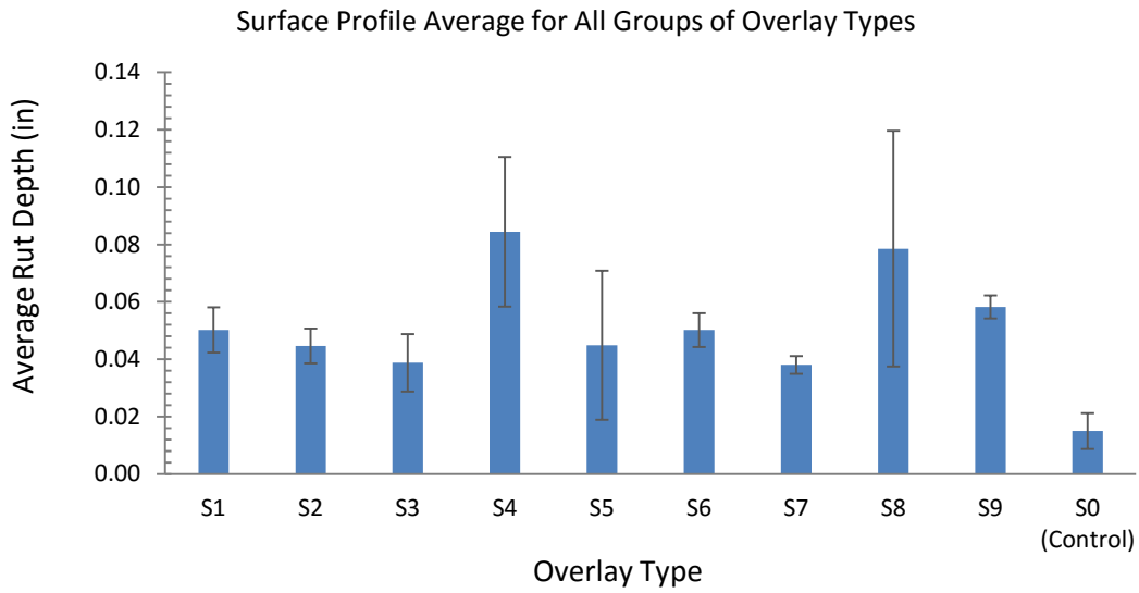
Figure 48. Surface profile average for all groups of overlay types.
