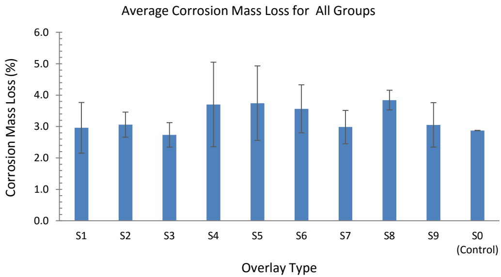
Figure 46. Average corrosion mass loss for all groups.
