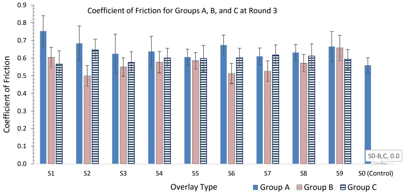
Figure 43. Coefficient of friction for groups A, B, and Cat Round 3.
