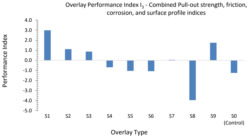
Figure 51. Overlay Performance Index ( I_3 ) - Including pull-out strength, friction, and corrosion indices.
