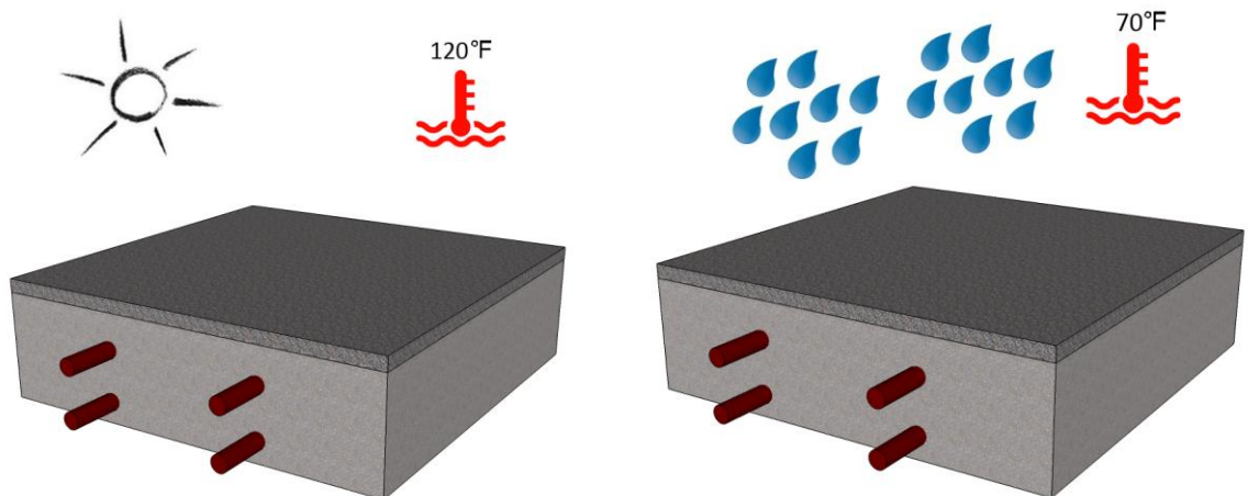
Figure 13. HURA test cycles: Heat and UV (left), rain and cool down (right).
