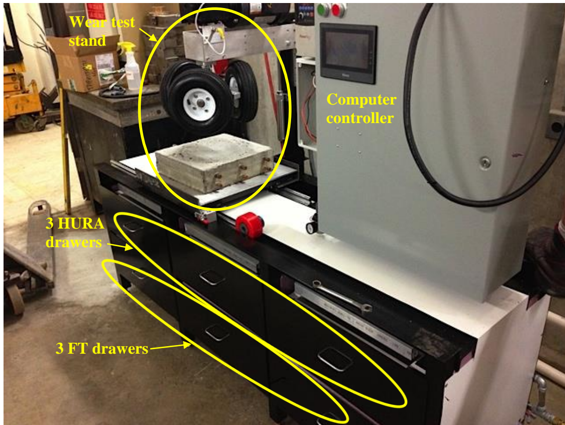
Figure 10. Automated computer-controlled machine for FT, HURA and wear testing of specimens.
