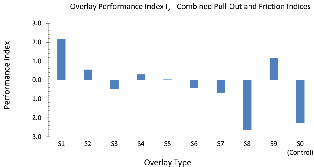
Figure 52. Overlay Performance Index ( I_2 ) - Including pull-out strength, and friction indices.
