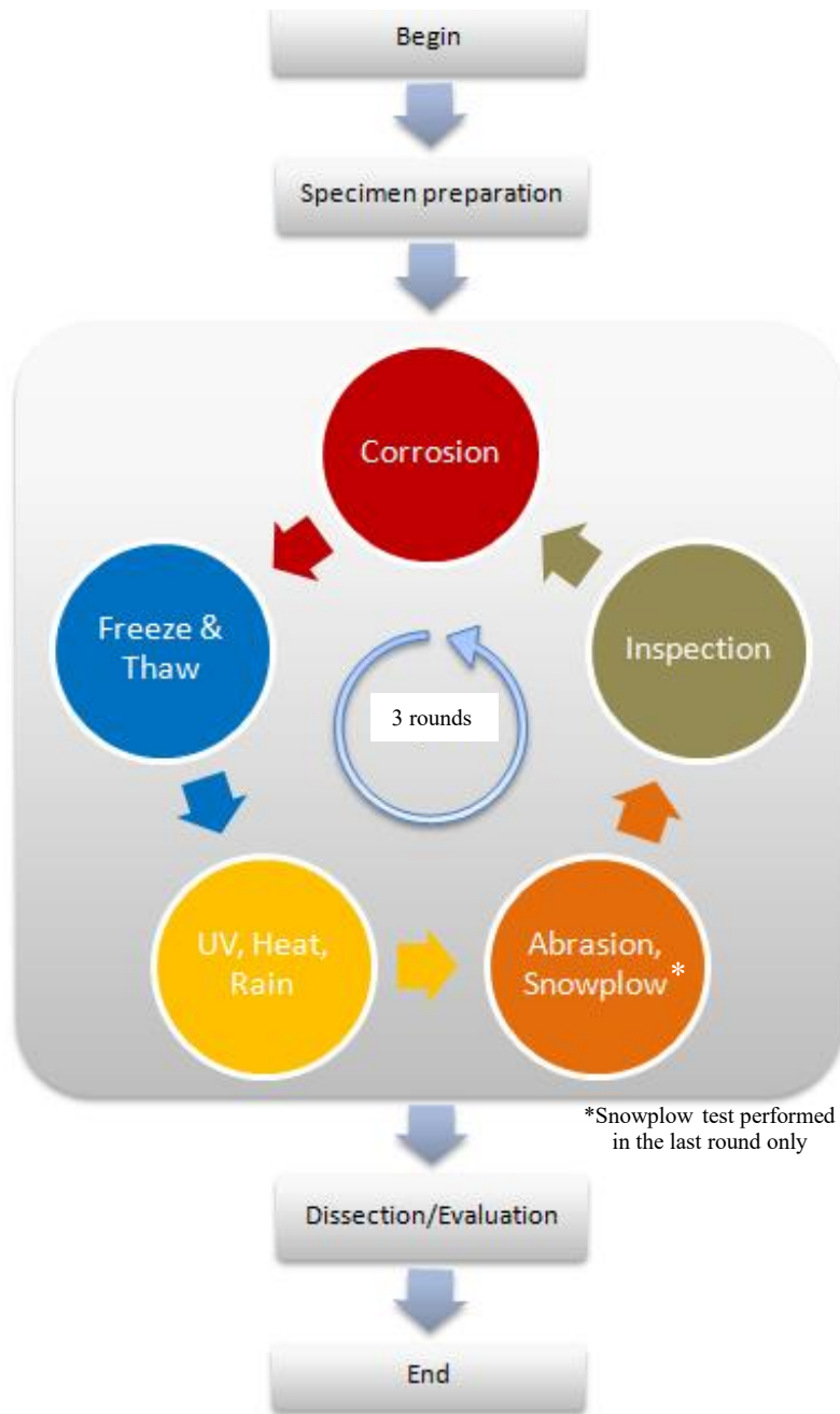
Figure 7. Test exposure cycles.
