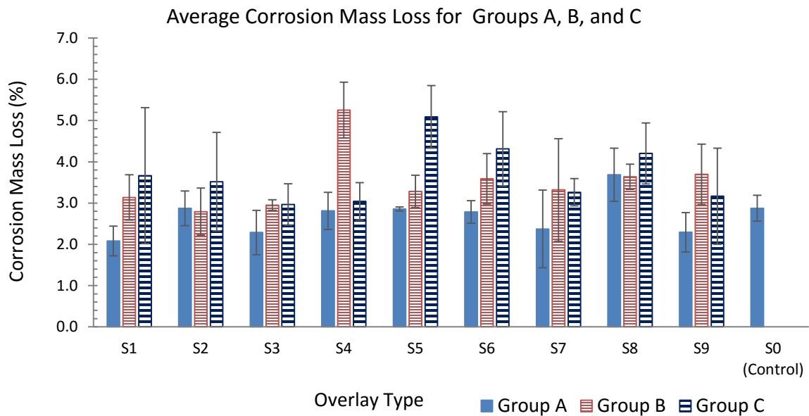
Figure 47. Average corrosion mass loss for Groups A, B, and C.
