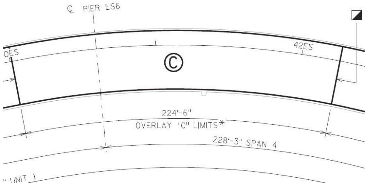
Figure 35. Section C drawing (from WisDOT).
