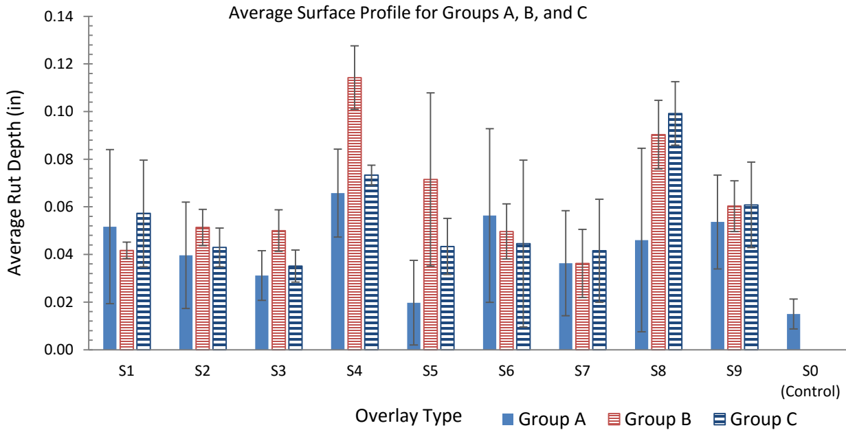
Figure 49. Average surface profile for groups A, B, and C.
