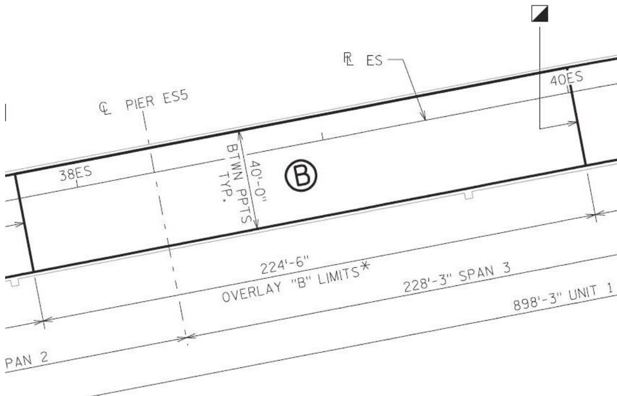
Figure 34. Section B drawing (from WisDOT).
