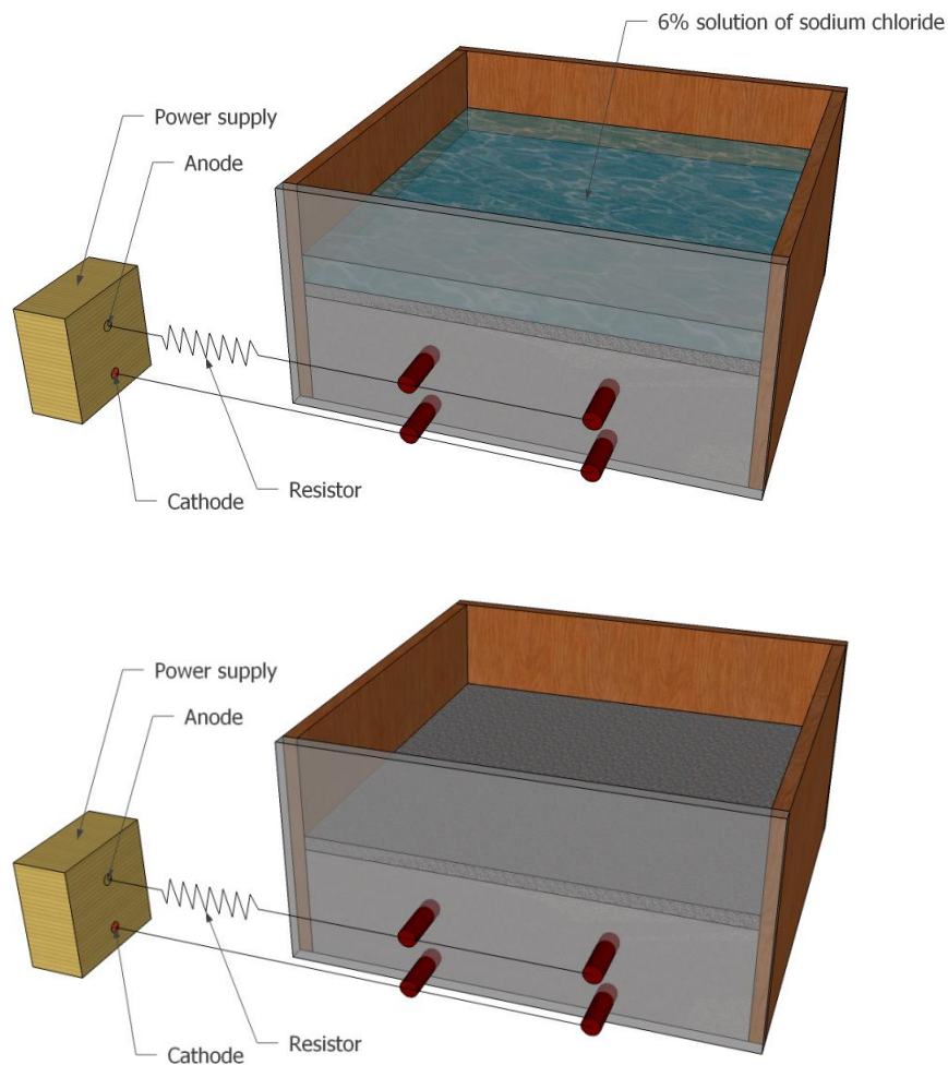
Figure 9. Accelerated corrosion exposure setup.
