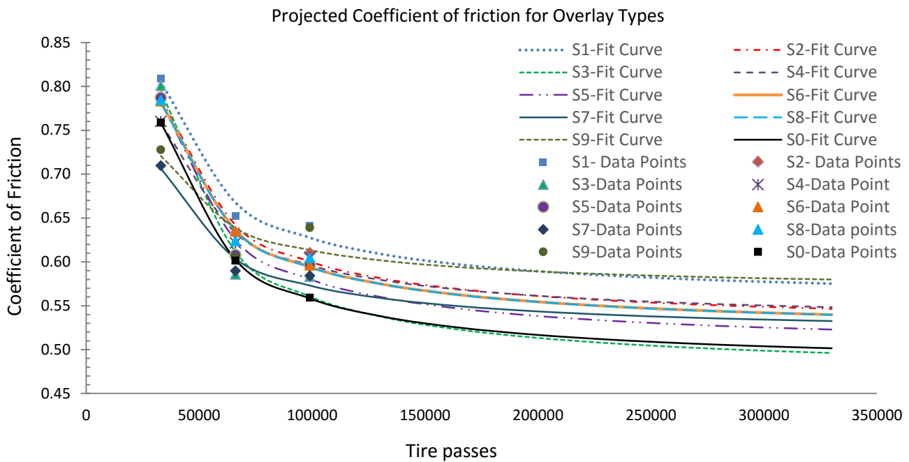
Figure 45. Projected coefficients of friction for various overlay types.
