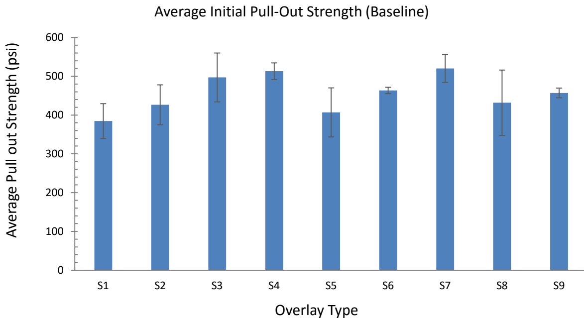
Figure 37. Average initial pull-out strength (baseline).
