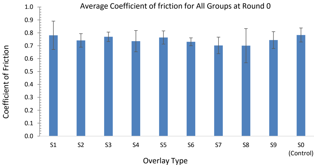
Figure 41. Initial average coefficients of friction for all groups at Round 0.
